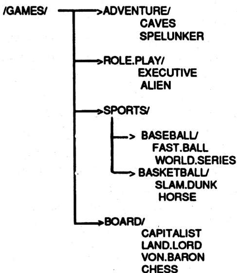
Figure 4-1 Hierarchical Structure
