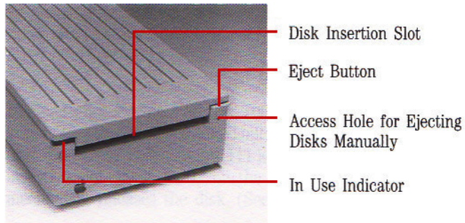
Figure 11. The Front of the UniDisk 3.5
