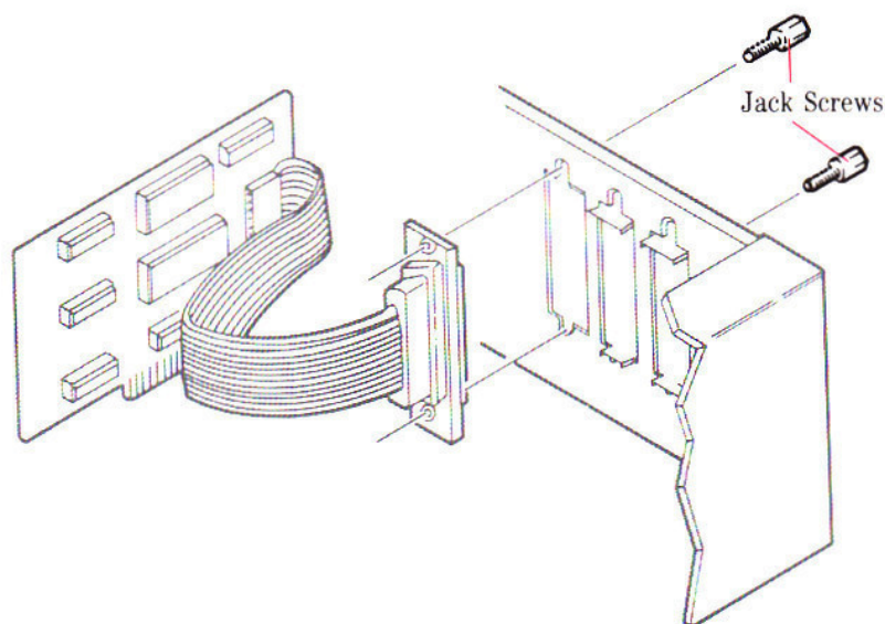
Figure 6. Arranging the Interface Card and Hardware
