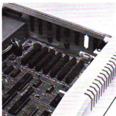
Figure 7. Card Slots
