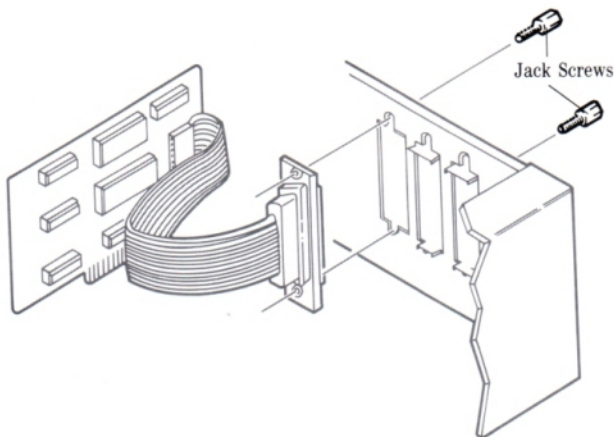
Figure 6. Arranging the Interface Card and Hardware
