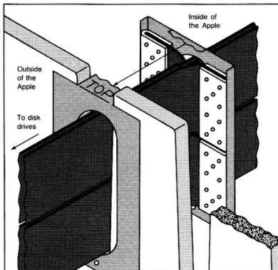
Figure 3-5. Position Four Cables in the Clamp
