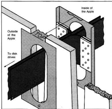
Figure 3-4. Position Two Cables in the Clamp
