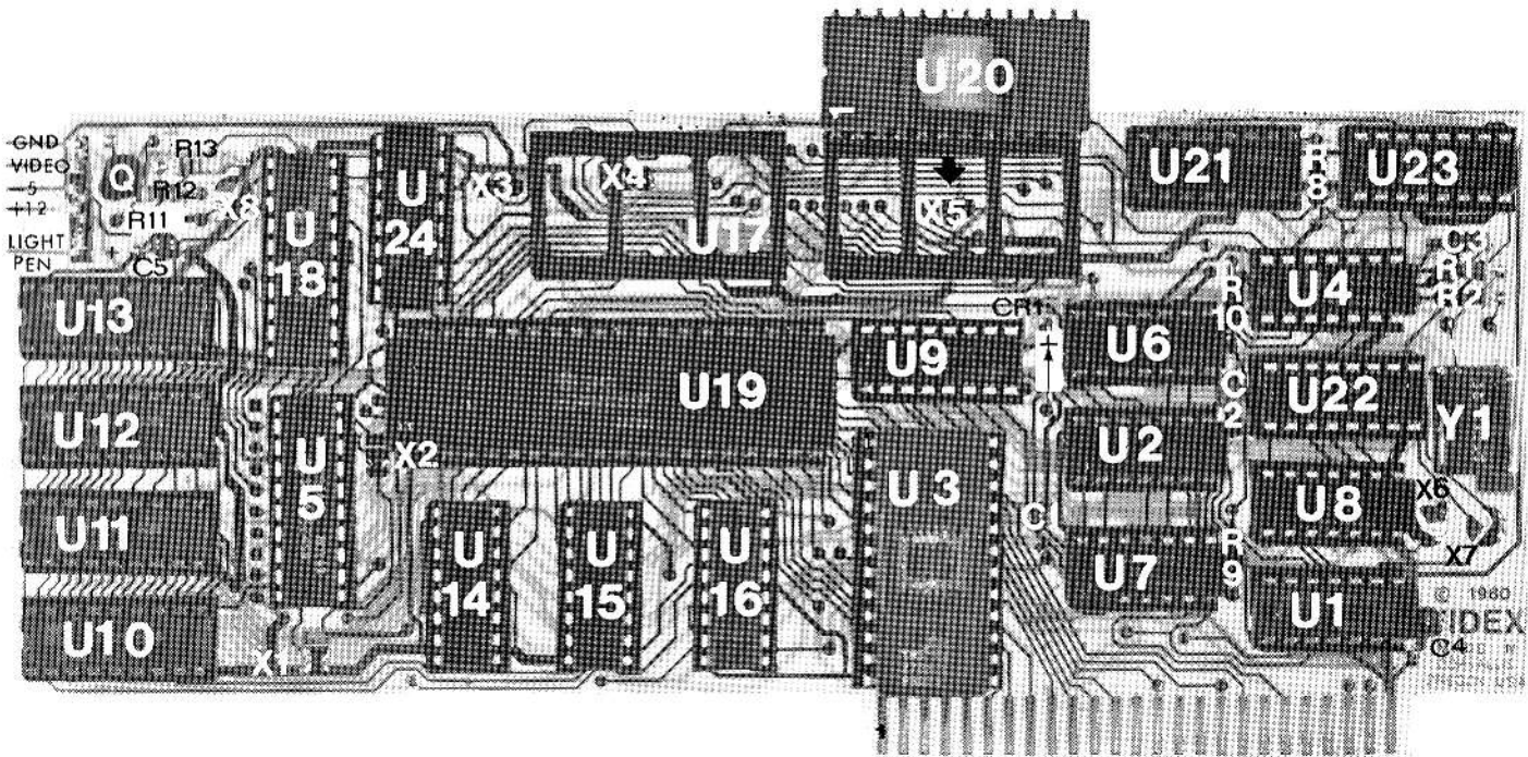
Figure 10: VIDEOTERM Board Photograph
