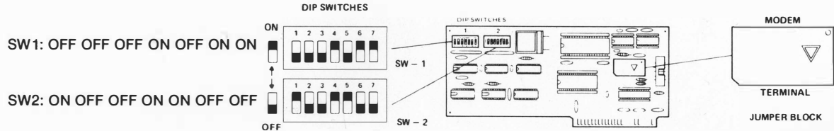
Figure 1-1. Super Serial Card Switches
