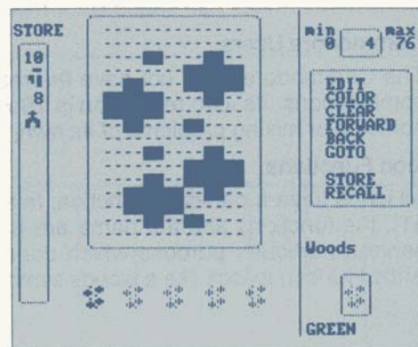
Fig 3.4 Graphic Editor
