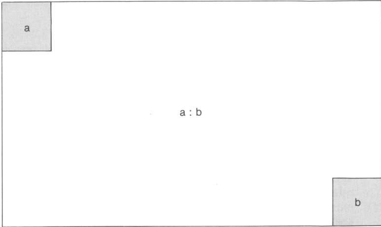
Figure 8.7. Range Reference
