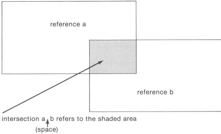
Figure 8.5. Intersection Reference
