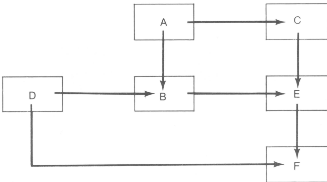
Figure 8.13. Dependency Diagram
