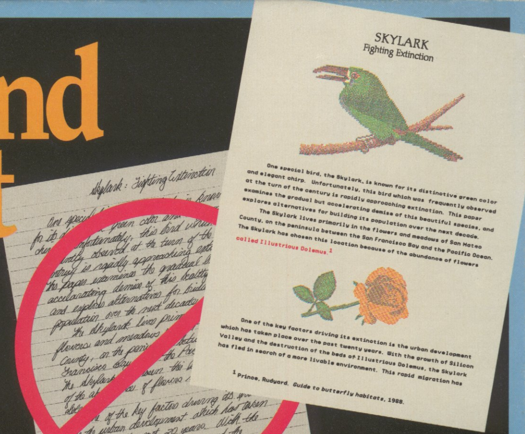
Page preview
