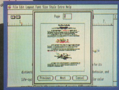
Multiple windows
