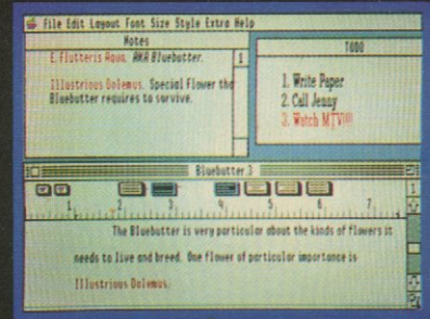
Multiple windows
