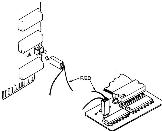
Figure 1-5 CPS Card 2-Pin Cable Installation
