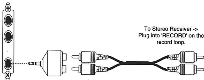
Connecting the SoundMeister to record from external stereo equipment using a RCA "Y" adaptor and patch cords..
