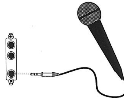
Connecting a microphone to the SoundMeister using a 3.5mm plug.
