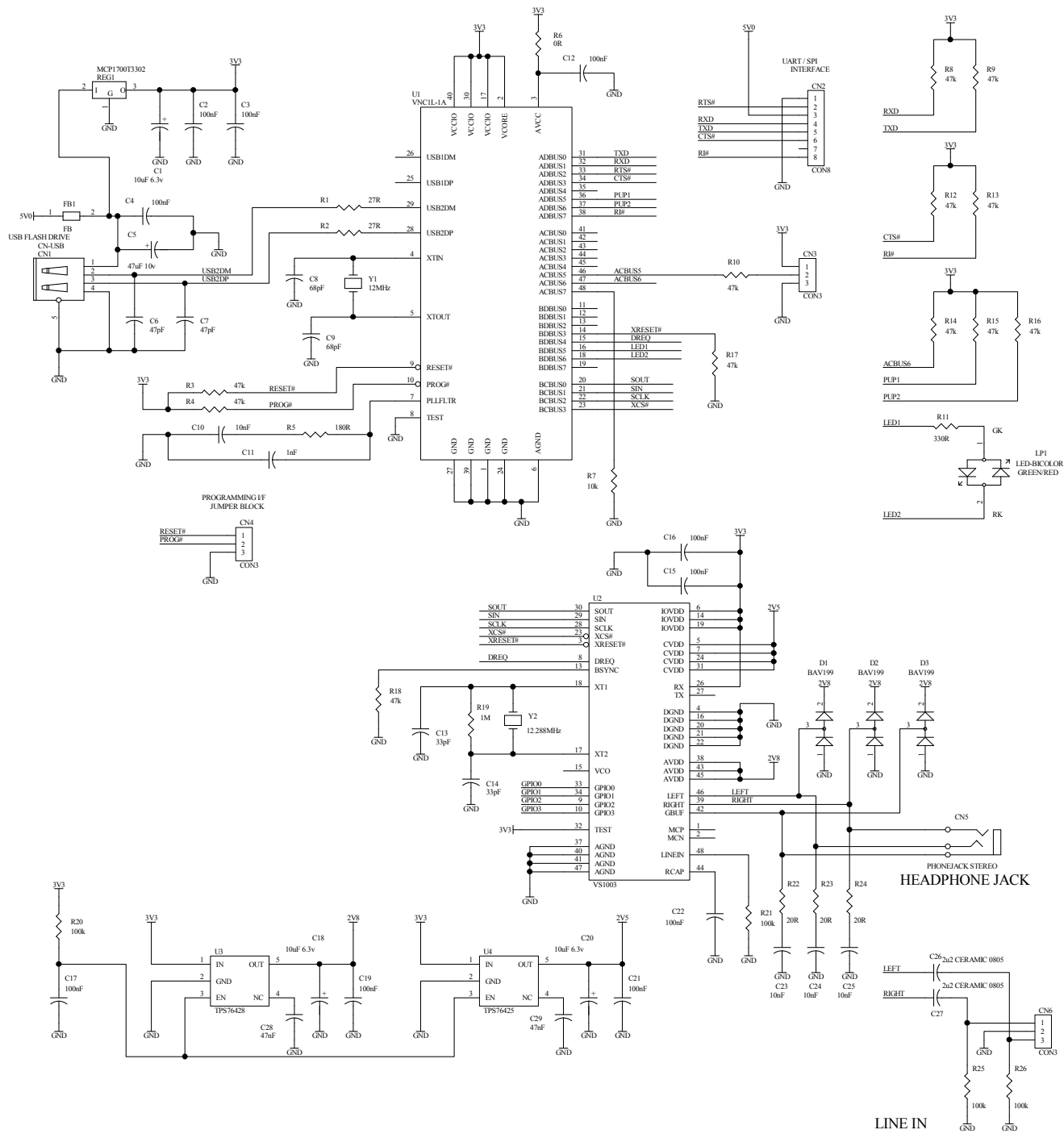
VINCULUM VMUSIC2 SCHEMATIC
