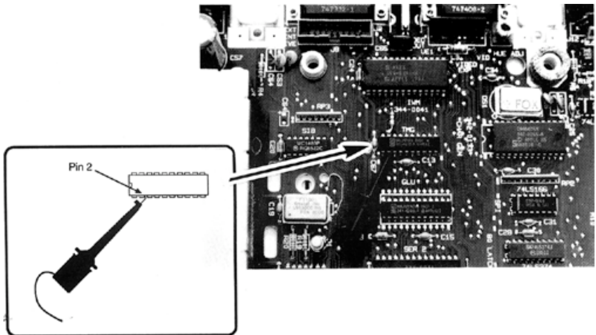
Figure 12: Fastening the Grabber Wire to the TMG chip
