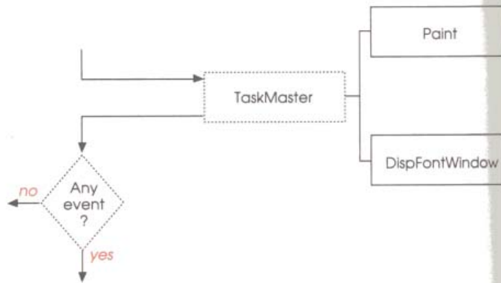
Figure 2-6 HodgePodge routines called by TaskMaster
