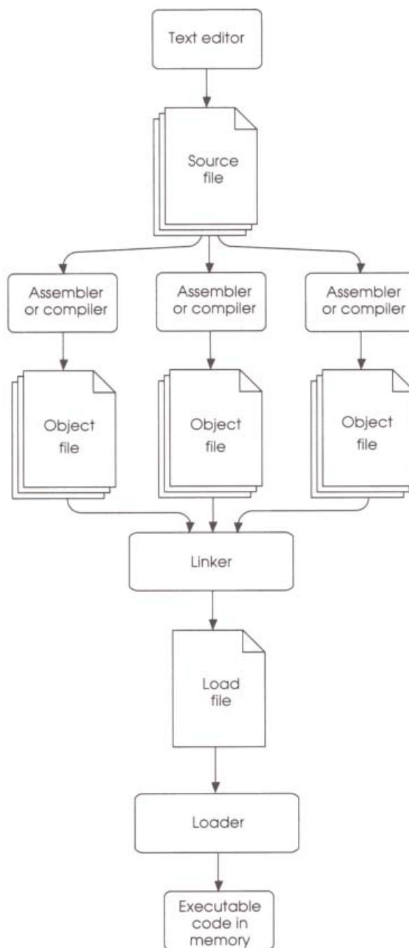
Figure 7-2 Creating an executable Apple Iks program
