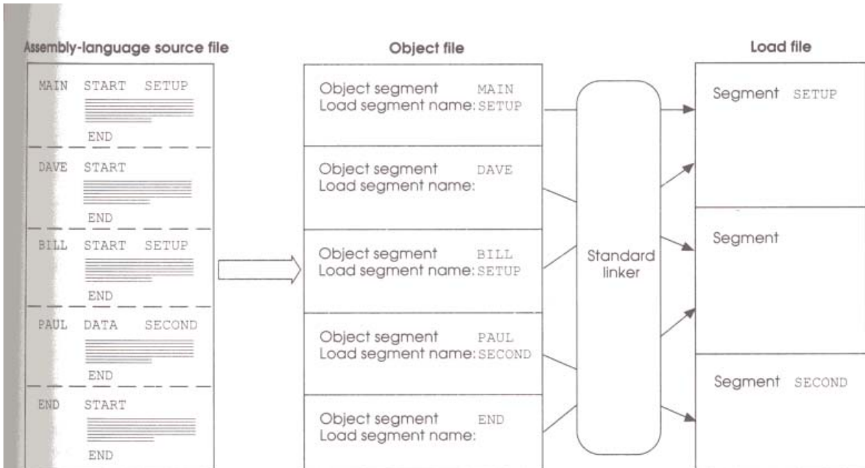
Figure 7-4 Assigning load segments in your source code
