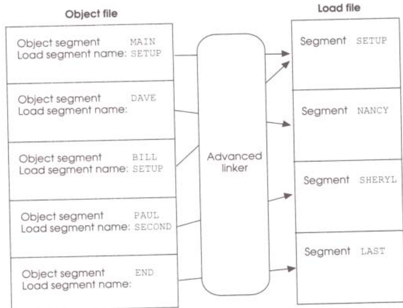
Figure 7-5 Assigning load segments with the advanced linker
