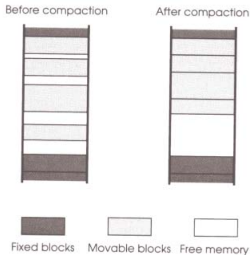
Figure 6-1 Memory fragmentation and compaction
